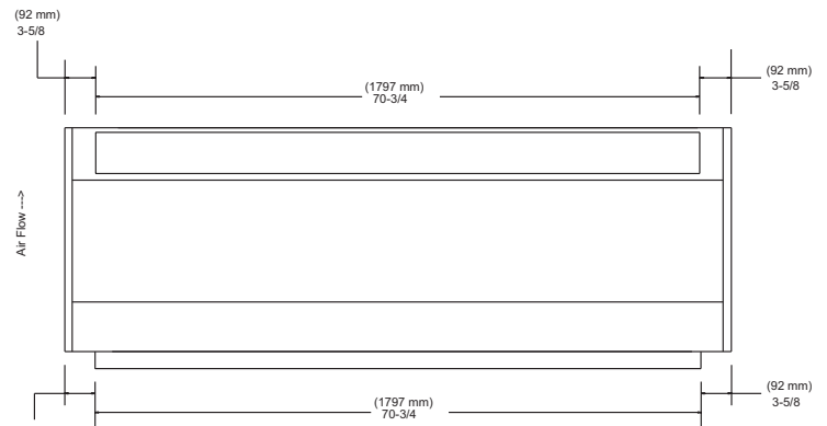
FRONT VIEW 78" (1981 mm) CABINET
