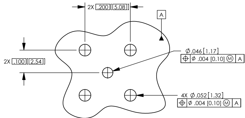
RECOMENDED PCB LAYOUT COMPONENT SIDE SHOWN
