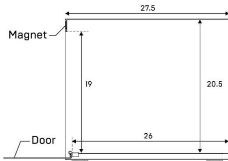
Side Sectional View • Door Open
