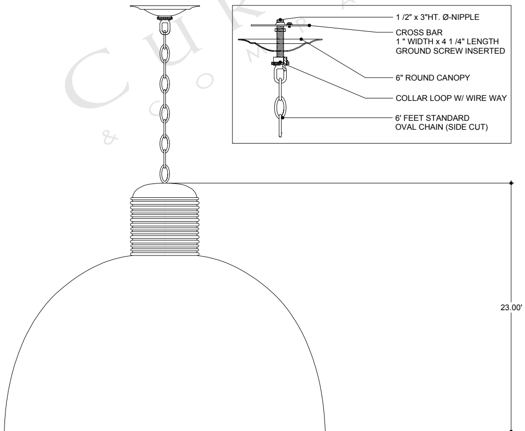
FRONT VIEW
