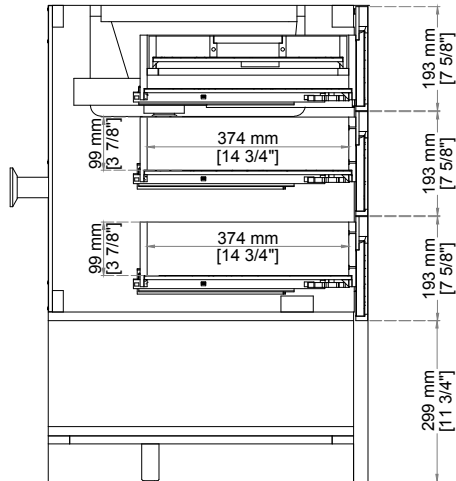
Side View 2
