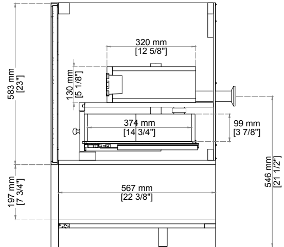
Side View 1
