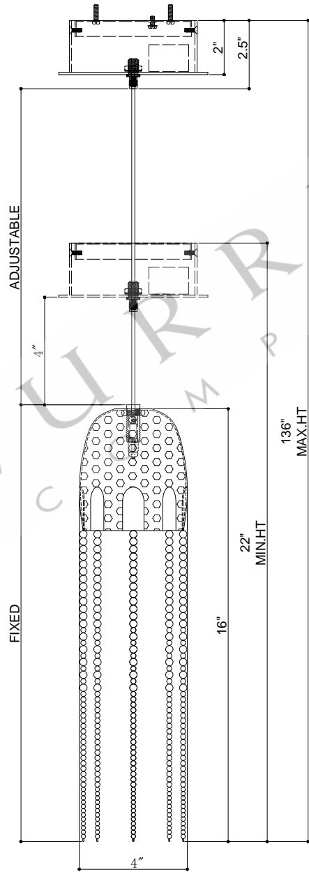
FRONT VIEW
