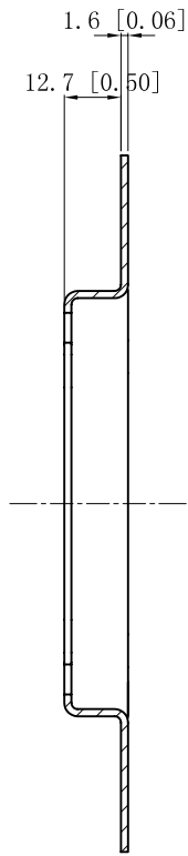
CUTAWAY VIEW A-A
