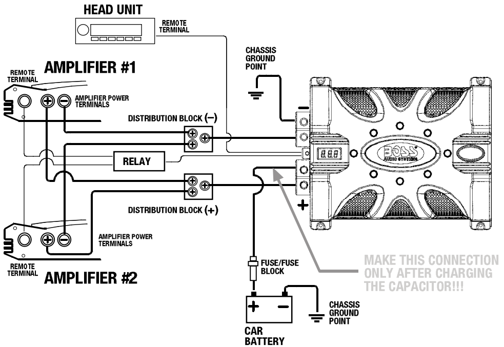
WIRING DIAGRAM: CAP20 or CAP35 In Two Amplifier System
