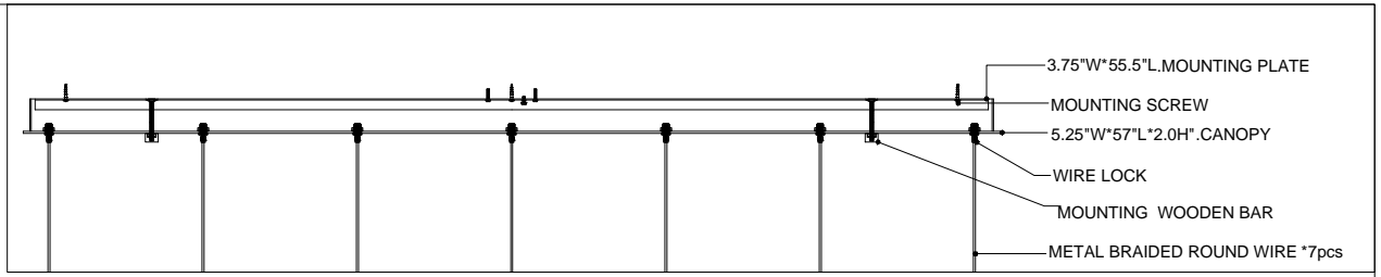
CANOPY DETAIL
