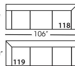
Large Seat End with Corner* L106" D40" H38" *available as right or left seated
