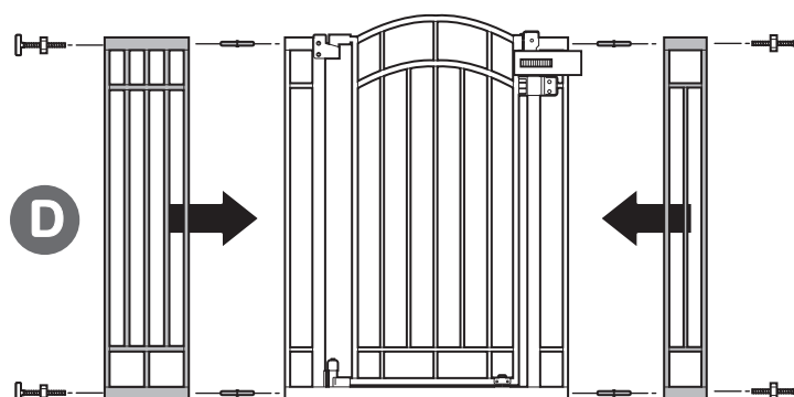
(41 in.- 44 in.) with one short and the long extension frames
