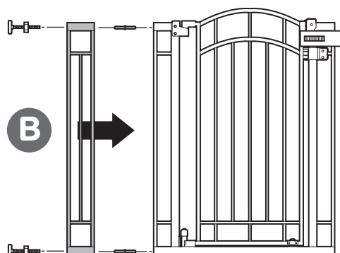
(33 in.- 36 in.) with one short extension frame
