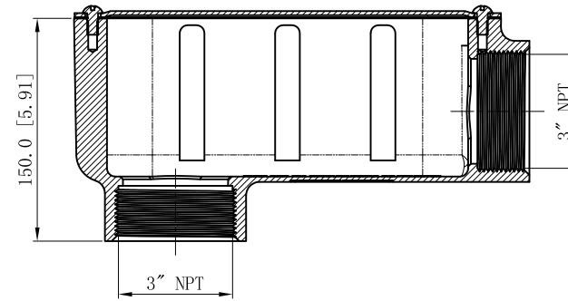
CUTAWAY VIEW A-A
