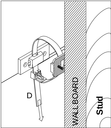
Secure to Stud behind Wallboard !
