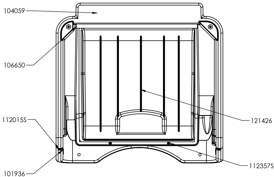
COVER ASSEMBLY
