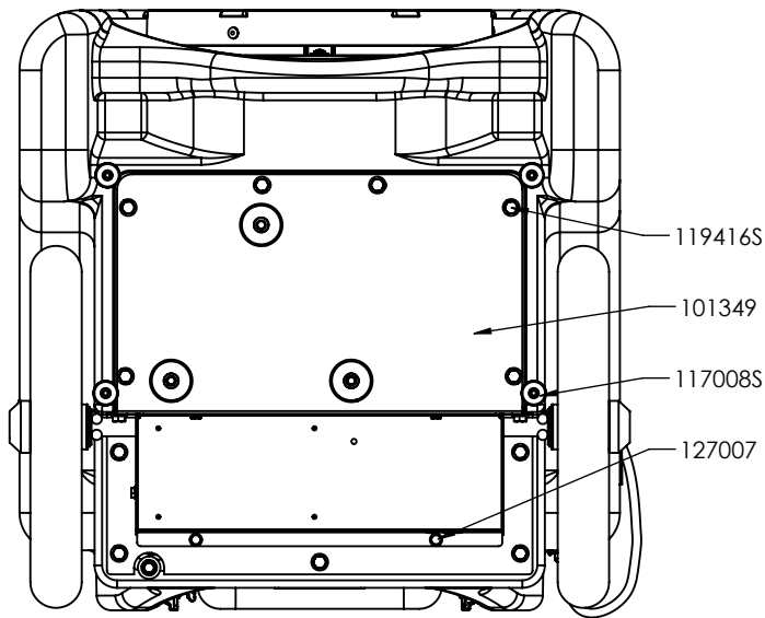
BOTTOM ASSEMBLY
