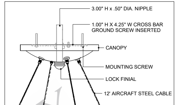
CANOPY DETAIL
