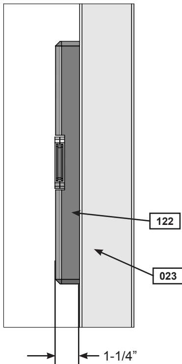
Fig. 12.9 Side View
