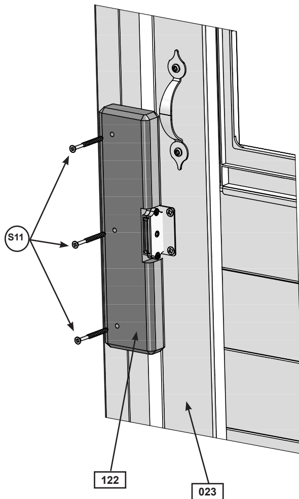
Fig. 12.8 Inside View
