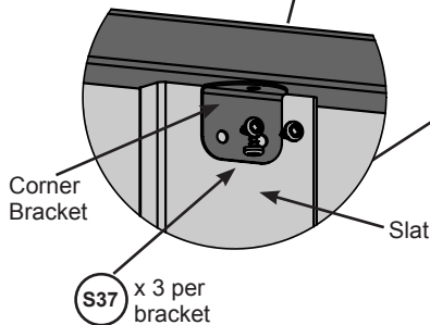
Fig. 6.2 Inside View
