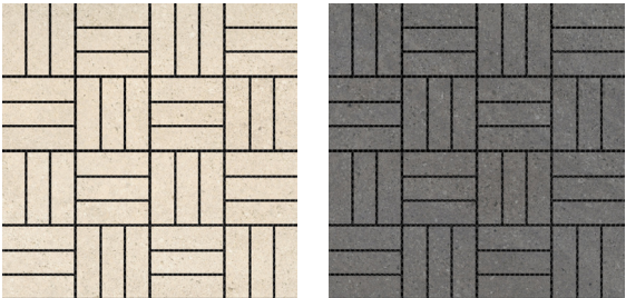
Mira Vega
