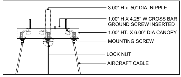
CANOPY DETAIL
