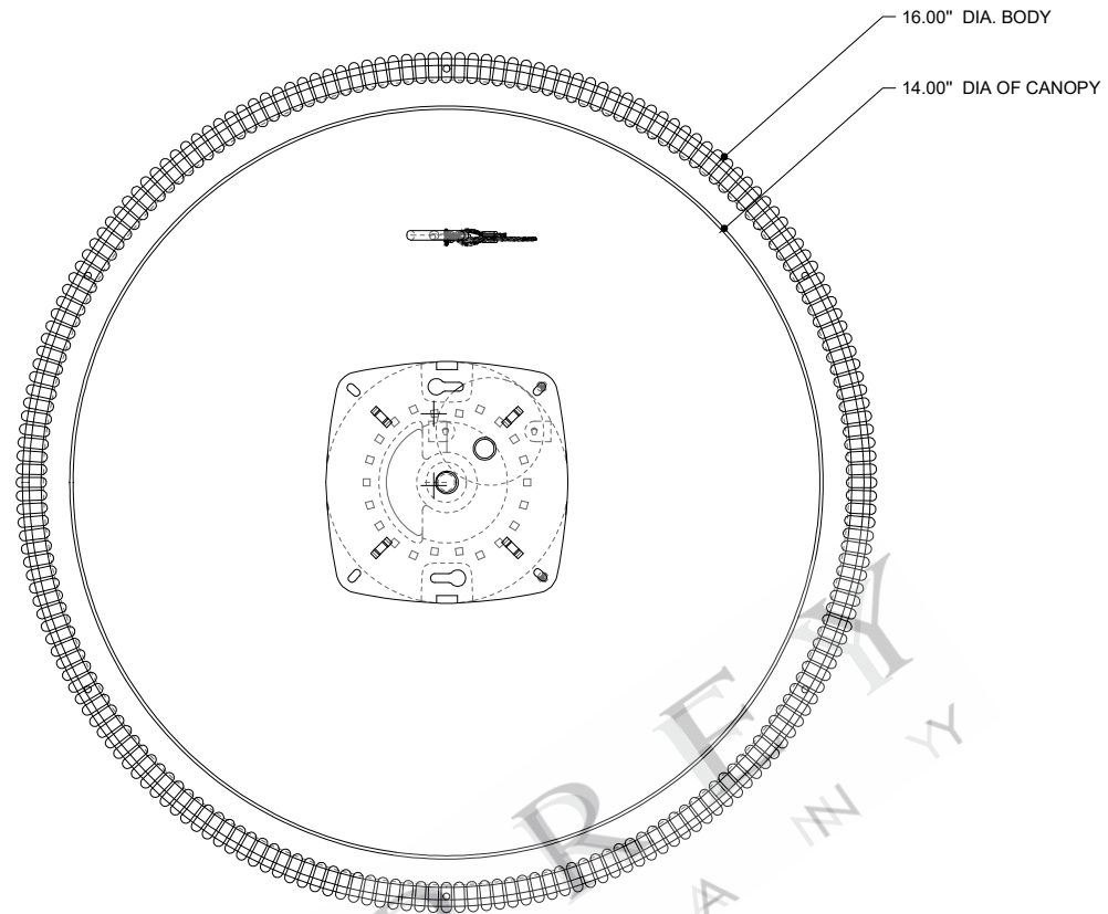
TOP VIEW
