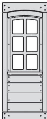
1pc. - [2718] Door Window Panel 1\frac{1}{4} \times 15\frac{3}{4} \times 40\frac{3}{4}'' Box 2 - 37602718B
