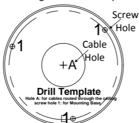
Figure 2-19 Drill Template
