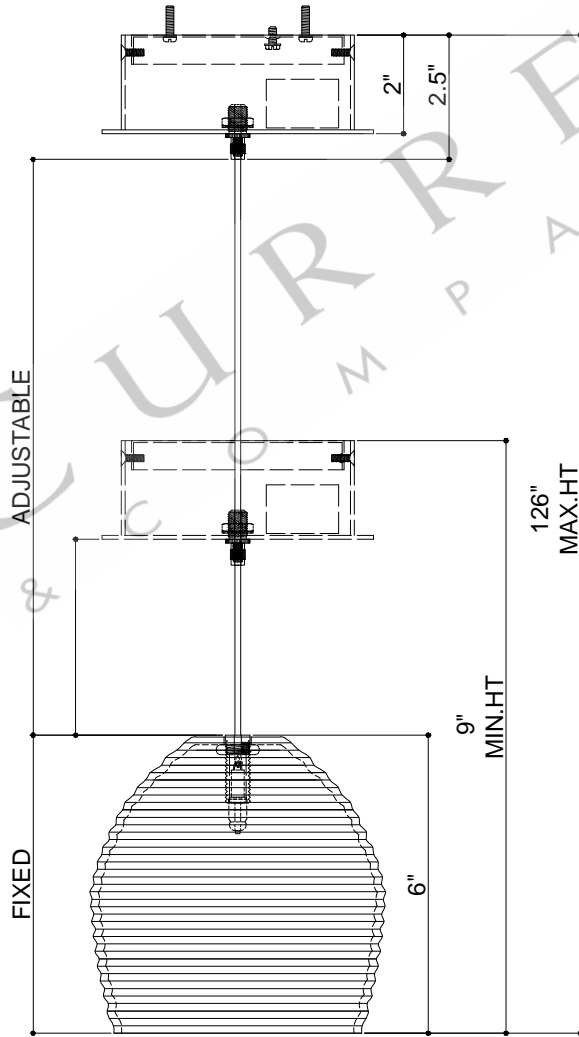
FRONT VIEW
