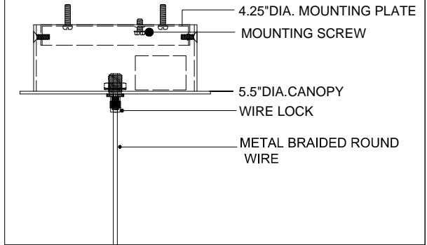
CANOPY DETAIL
