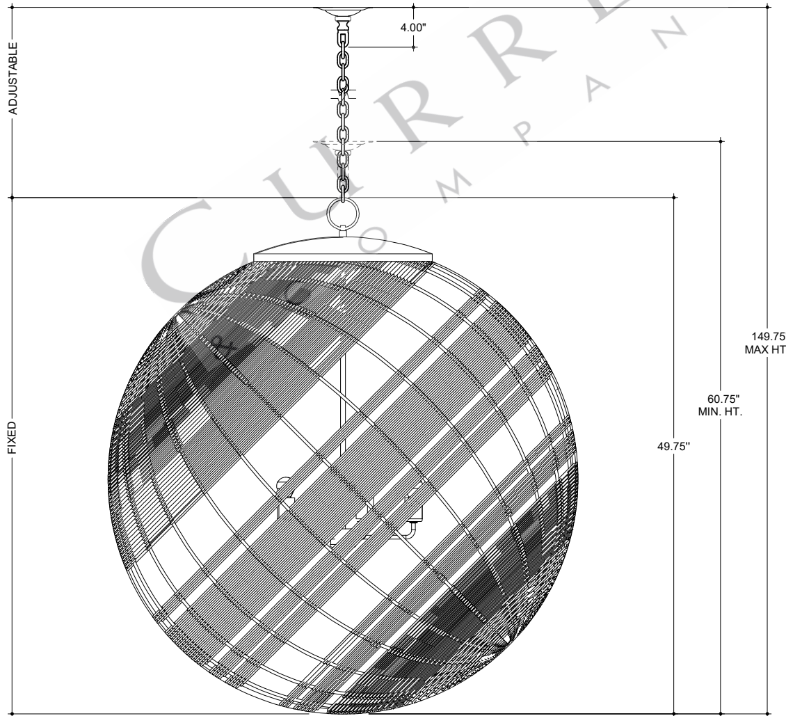
FRONT VIEW
