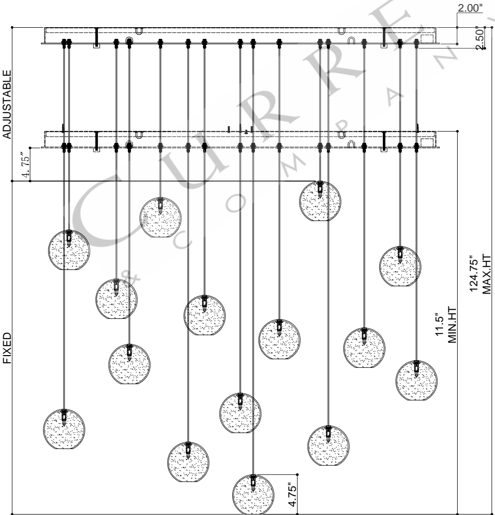
FRONT VIEW
