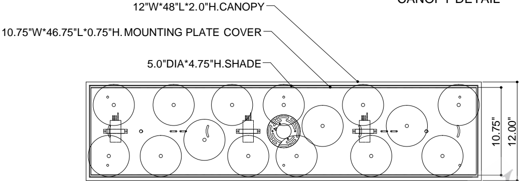
CANOPY DETAIL
