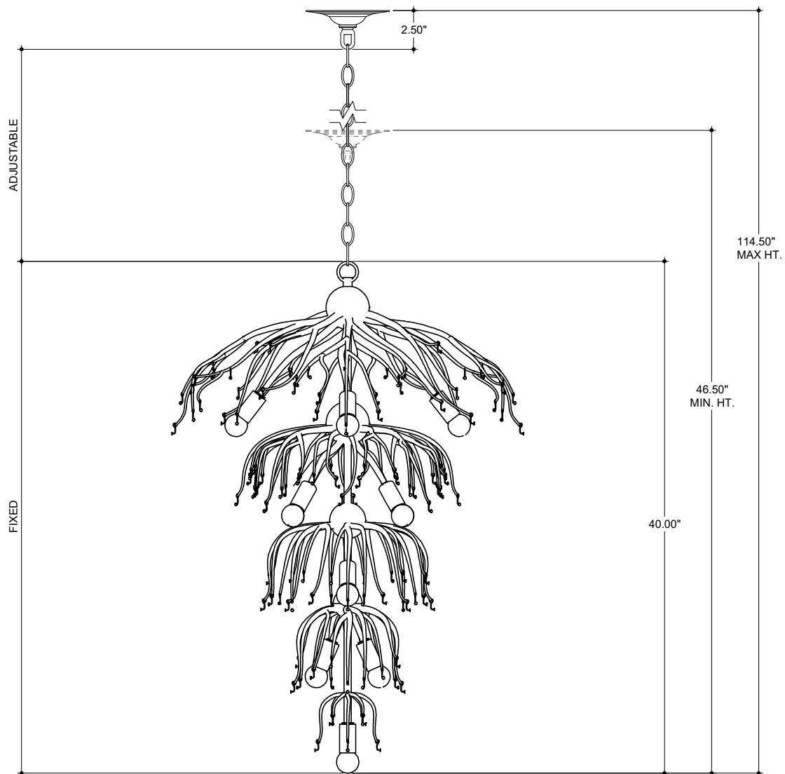
FRONT VIEW
