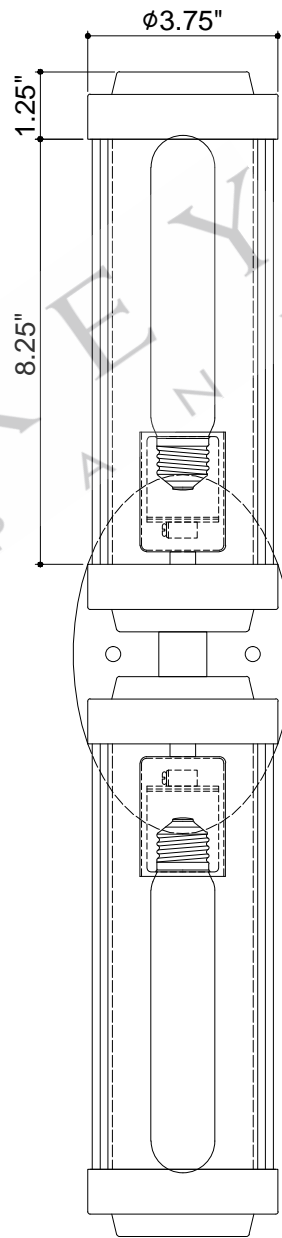
FRONT VIEW
