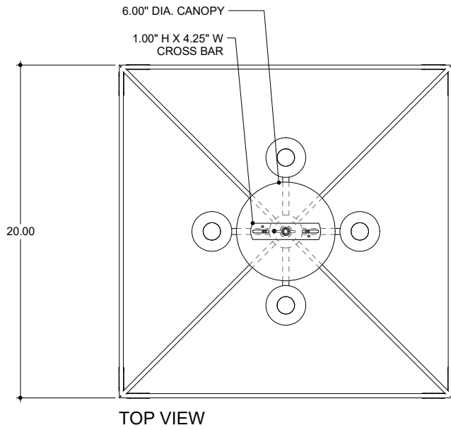
CANOPY DETAIL
