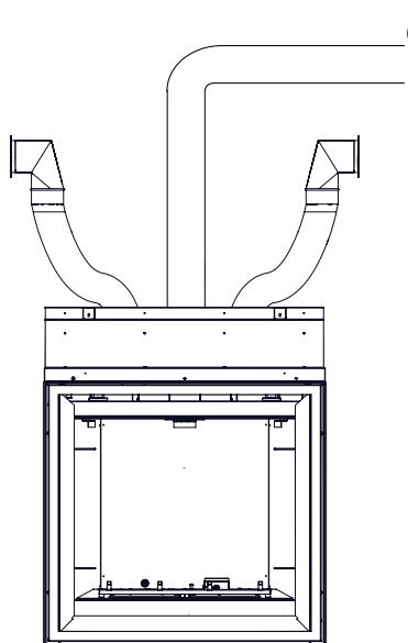
Side Termination
