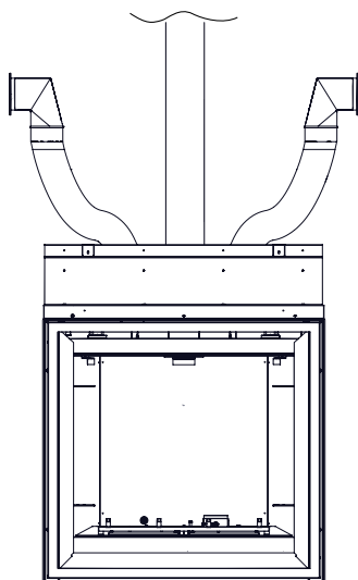
Rear / Top Termination
