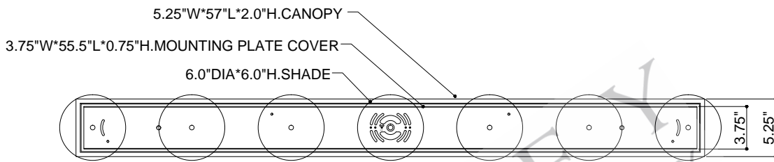
TOP VIEW
