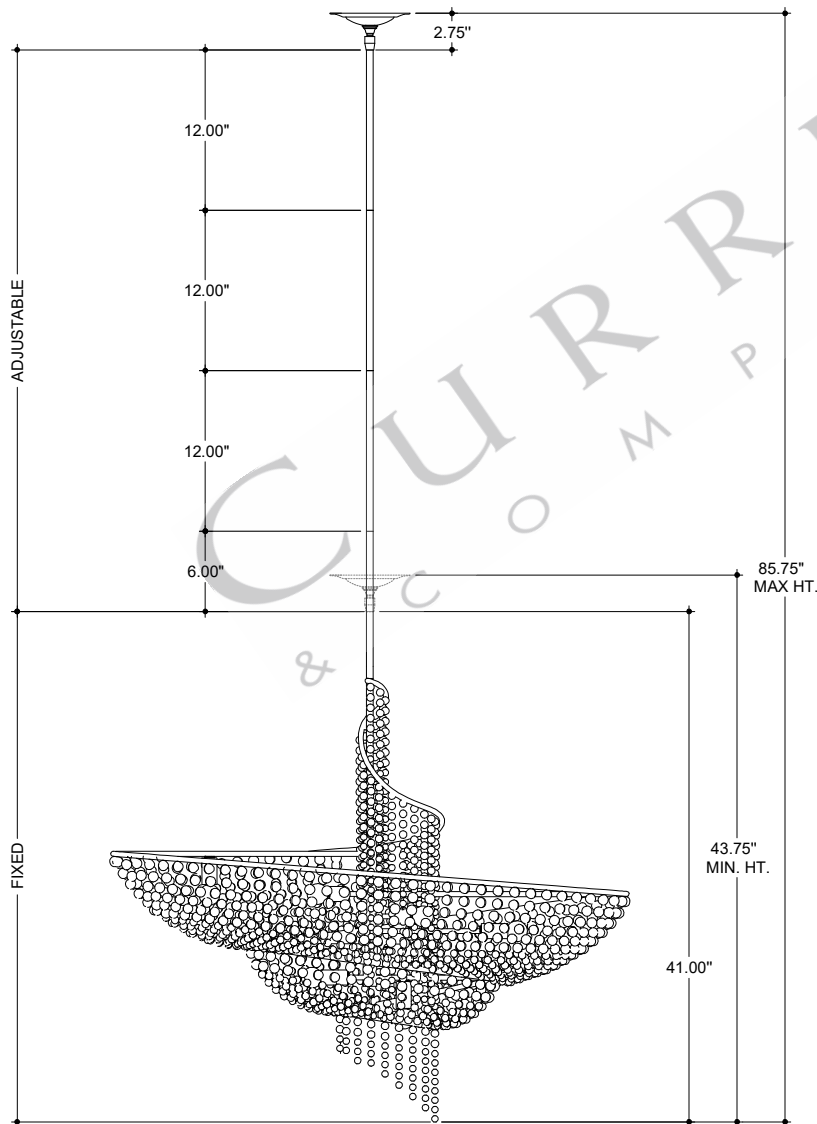
FRONT VIEW
