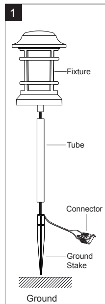
Fixture Assembly
