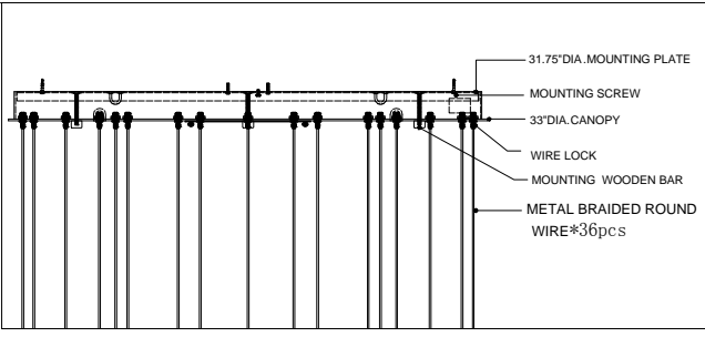
CANOPY DETAIL
