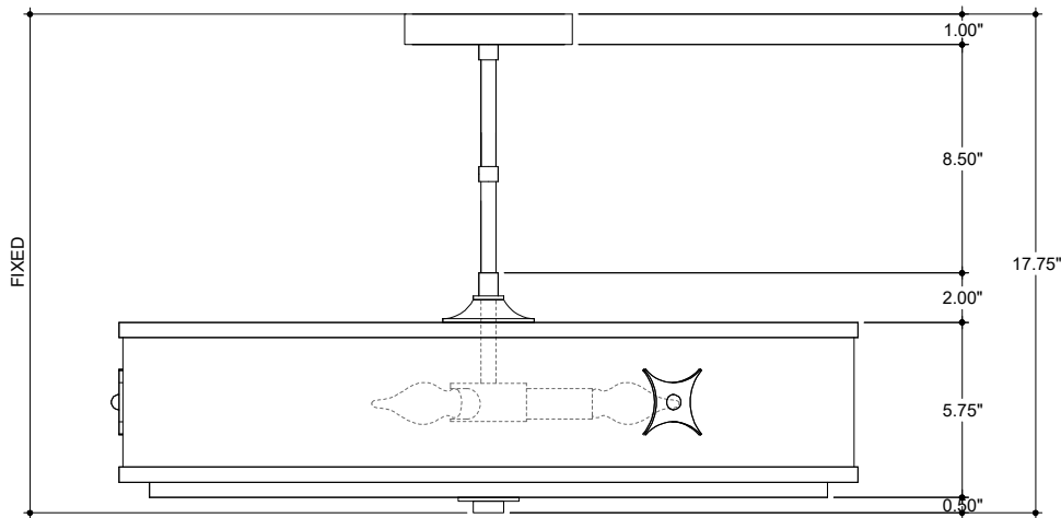
FRONT VIEW
