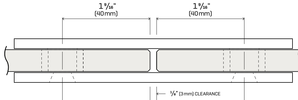
TEMPLATE FOR 180° GLASS-TO-GLASS INSTALLATION
