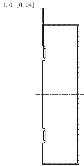
CUTAWAY VIEW A-A
