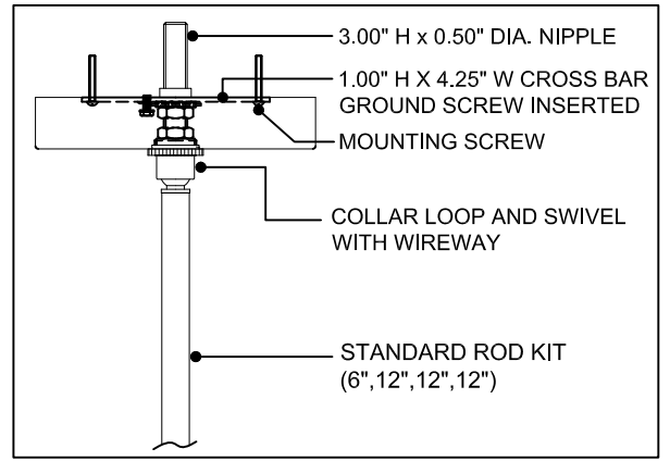
CANOPY DETAIL
