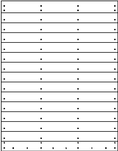
(1) 351 - 1-1/4 x 39 x 50-7/16" Roof Panel B - 37599029
