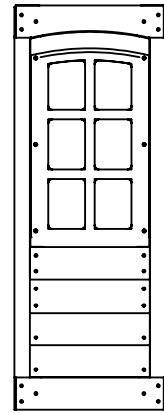
(1) 120 - 1-1/4 x 15-3/4 x 42-1/8" Door Window Panel 37608977
