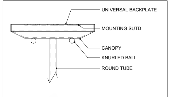
CANOPY DETAIL
