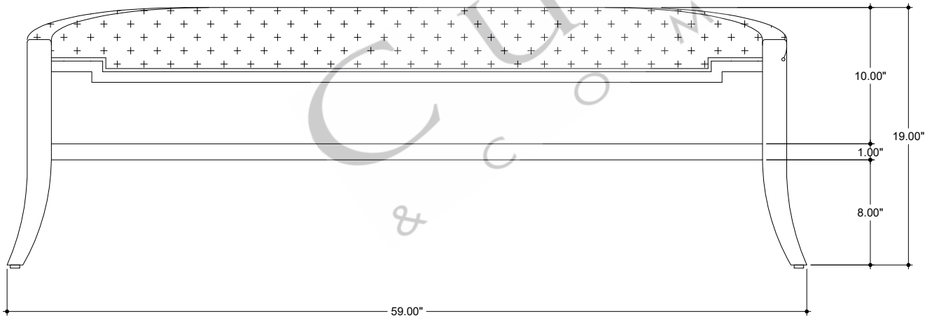
FRONT VIEW
