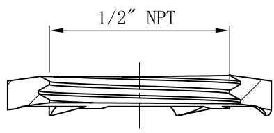
CUTAWAY VIEW A-A
