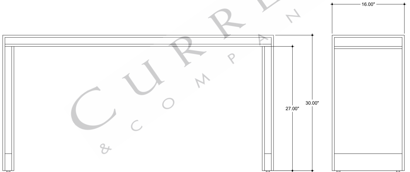
FRONT VIEW
