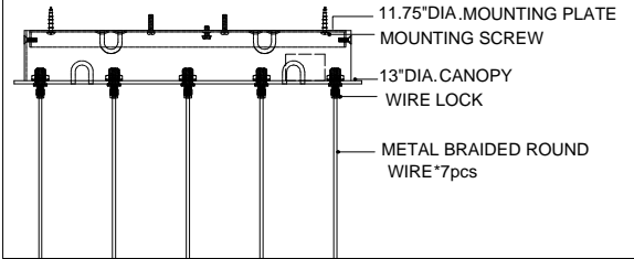
CANOPY DETAIL
