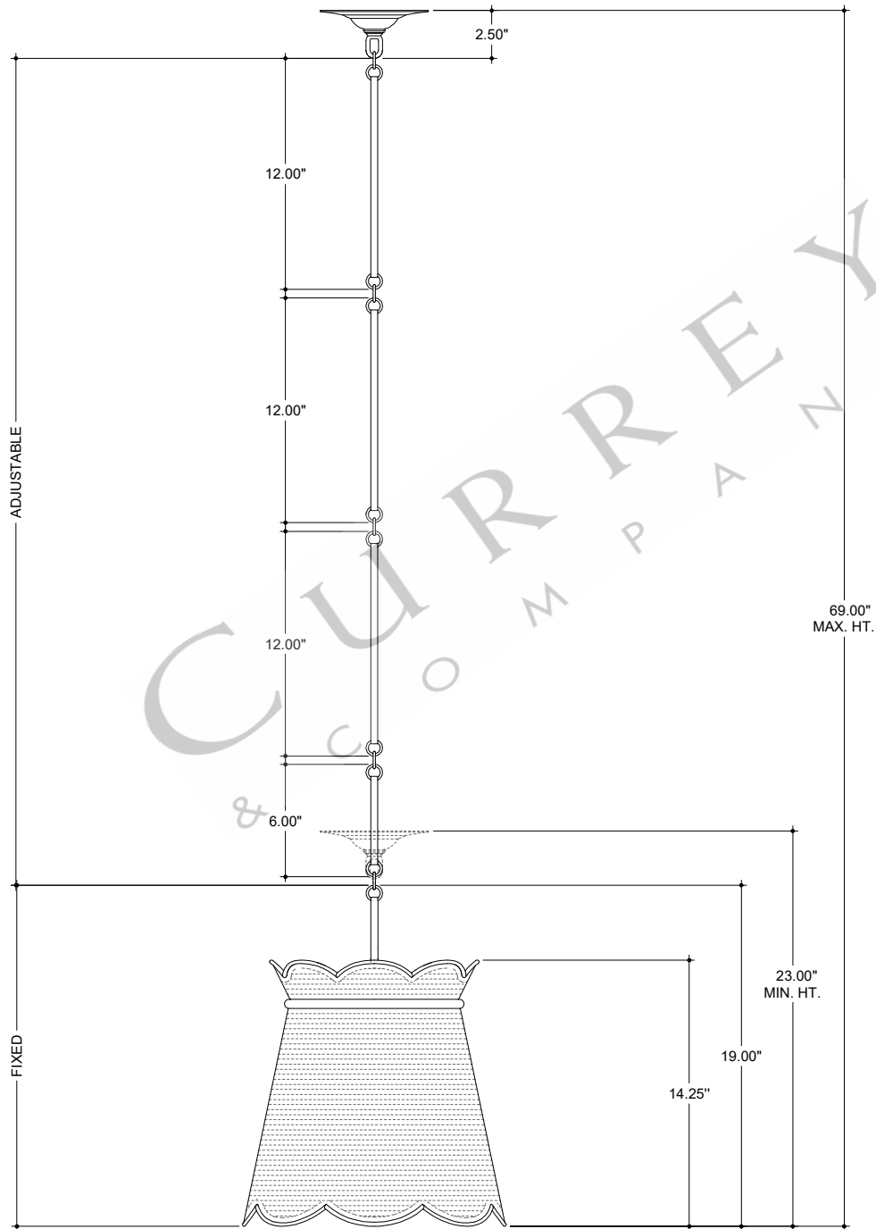
FRONT VIEW
