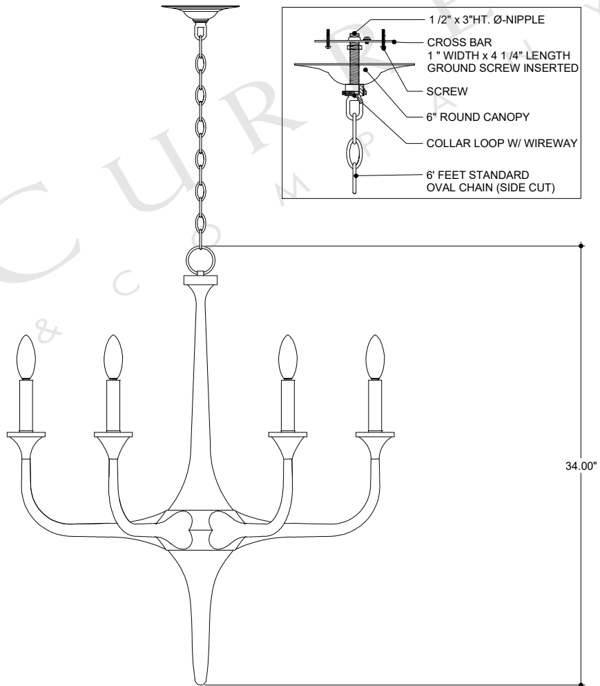
FRONT VIEW
