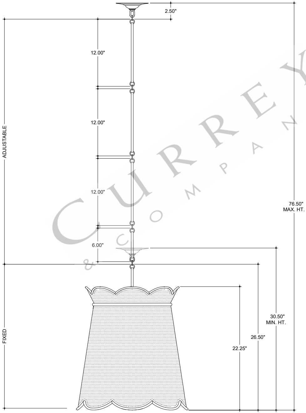
FRONT VIEW
