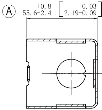
CUTAWAY VIEW A-A
