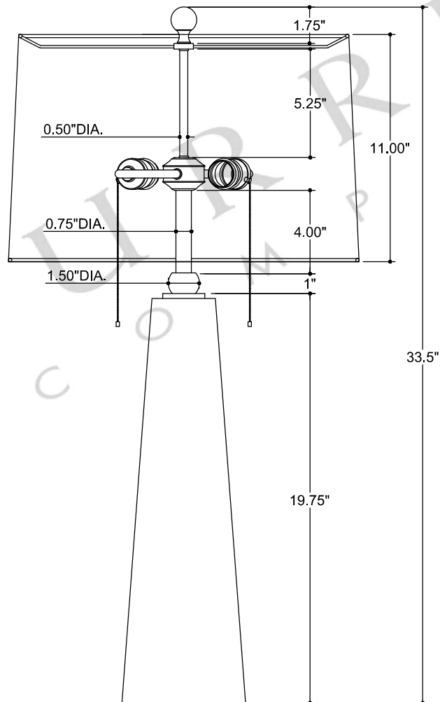
FRONT VIEW
