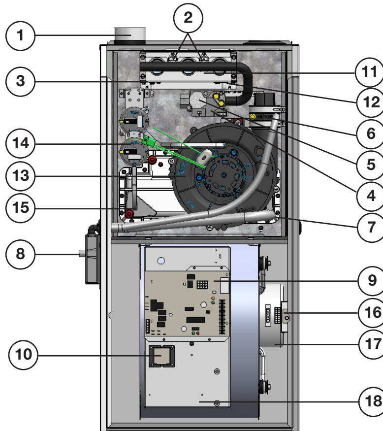
FIGURE 1 - FURNACE COMPONENTS
