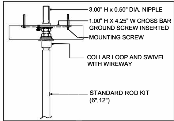
CANOPY DETAIL
