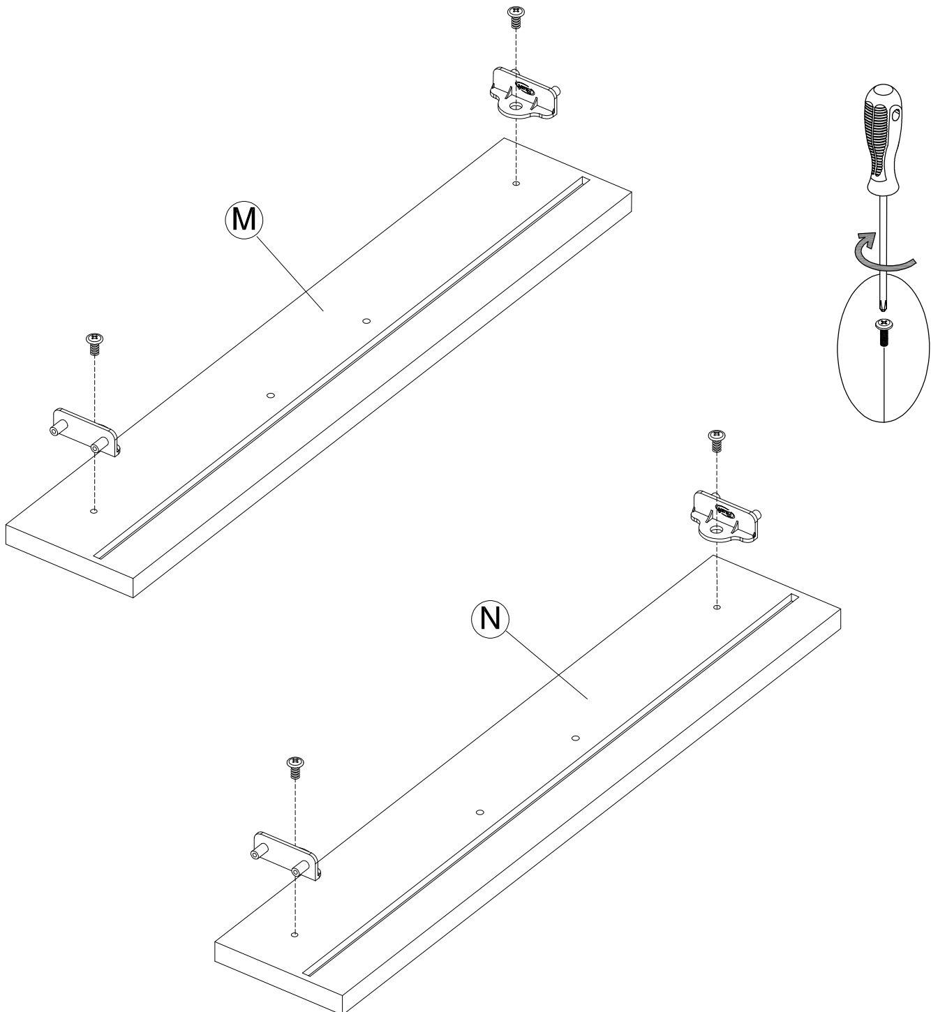
Drawer Bracket
